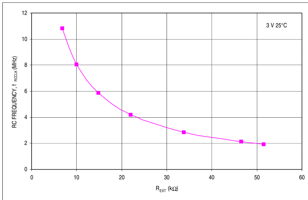
Figure 16-8. RC versus Frequency (3 Volts @ 25°C)
