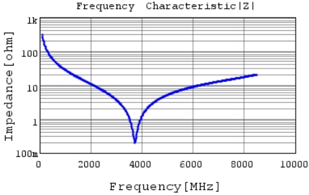
GJM1555C1H5R3WB01 |Z| DC0V, 25degC
