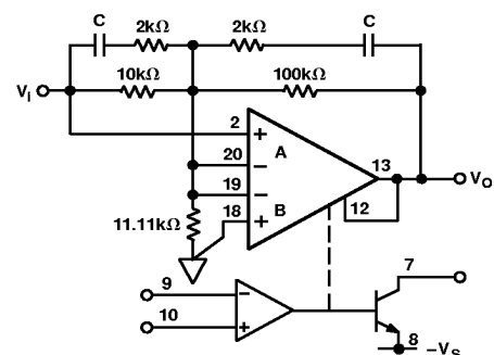
Figure 15. AD630 with External Feedback
