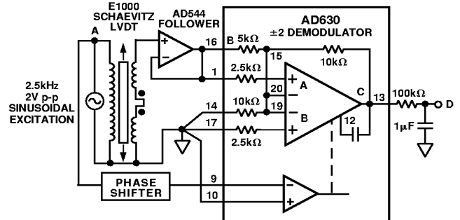
Figure 20. LVDT Signal Conditioner
