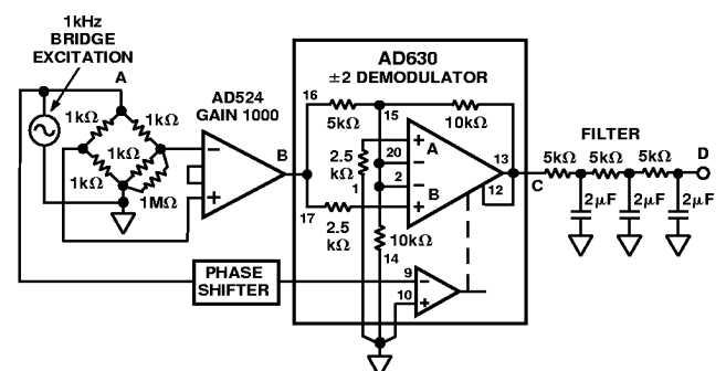
Figure 21. AC Bridge System
