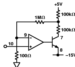
Figure 16. Comparator Hysteresis
