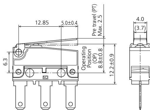
External dimensions
