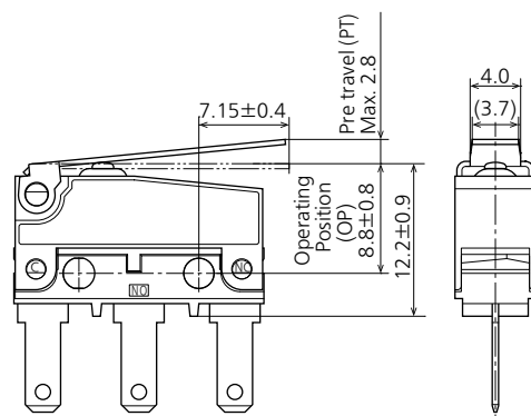
External dimensions
