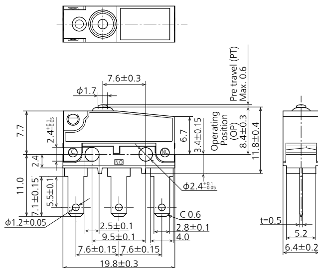
External dimensions
