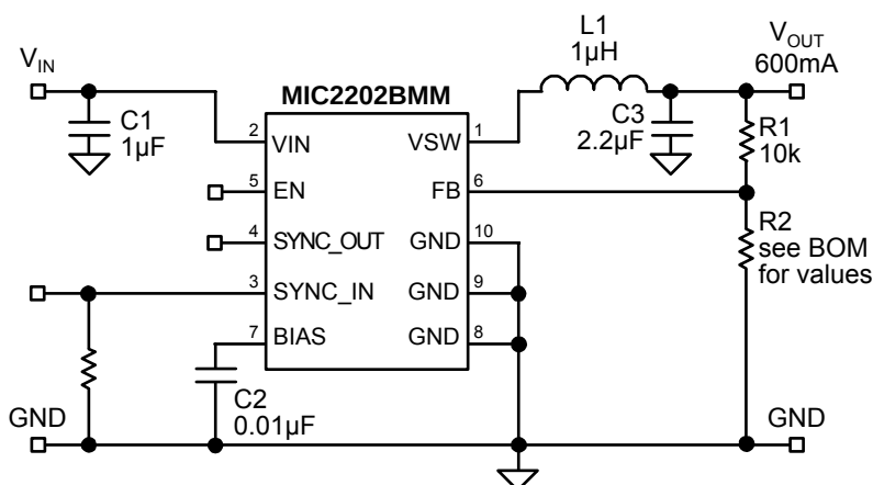
Figure 7. MIC2202BMM Schematic
