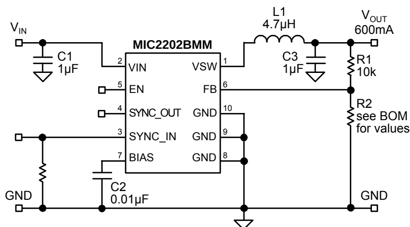
Figure 8. MIC2202BMM Schematic
