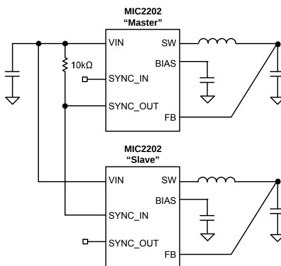
Figure 4. Master-Slave Operation
