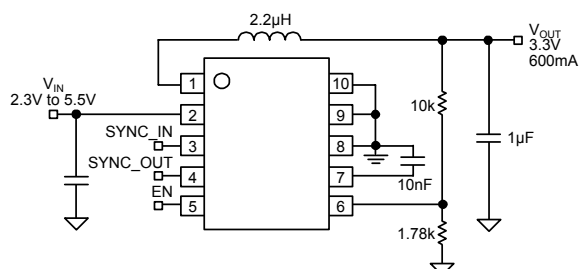
Adjustable Output Synchronous Buck Regulator
