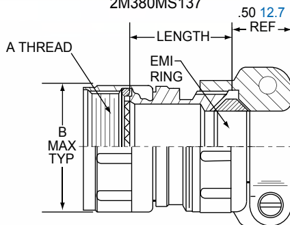
STRAIGHT ENTRY ROTATABLE COUPLING 2M380MS137
