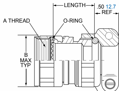
45° ENTRY ROTATABLE COUPLING 2M370MB038
