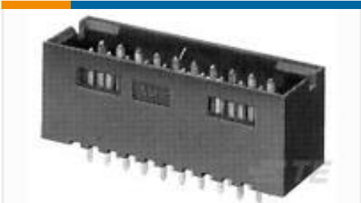
TE Part #6-103169-2 28 MODII HDR DRST SHRD .100CL
