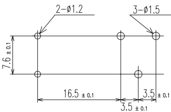
DRILLING DIAGRAM(2/1) (BOTTOM VIEW)
