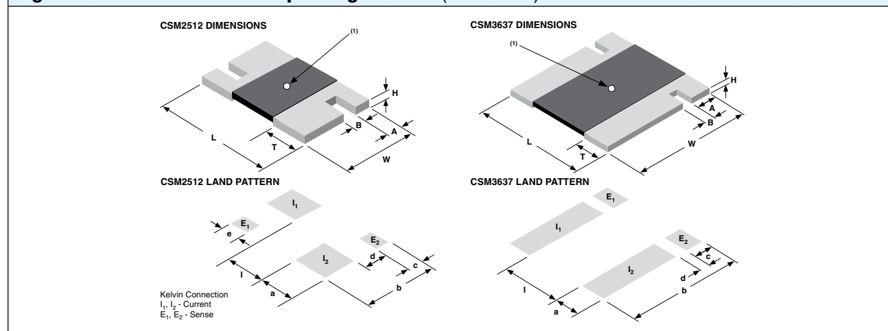
Figure 2 – Dimensions and Imprinting in inches (millimeters)
