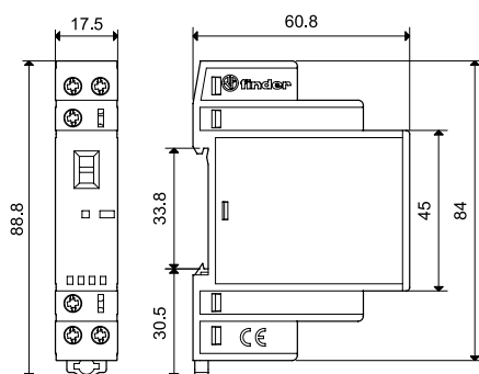
Type 22.32 Box clamp
