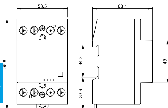
Types 22.44/22.64 Box clamp
