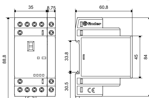
Types 22.34 + 022.33/022.35 Box clamp
