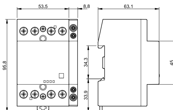
Types 22.44/22.64 + 022.63/022.65 Box clamp
