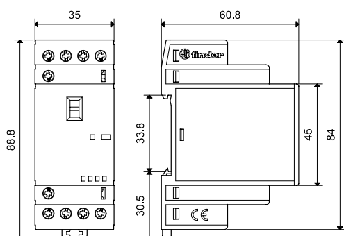
Type 22.34 Box clamp
