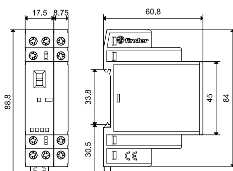
Types 22.32 + 022.33/022.35 Box clamp
