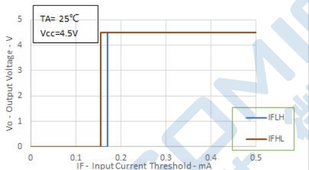
Fig.5 Input Current vs. Voltage
