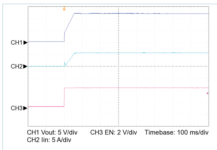
Figure 17 — Startup from EN, V_{IN} = 30\text{ V} , C_{OUT\_EXT} = 10000\text{ μF} , R_{LOAD} = 0.896\text{ Ω}
