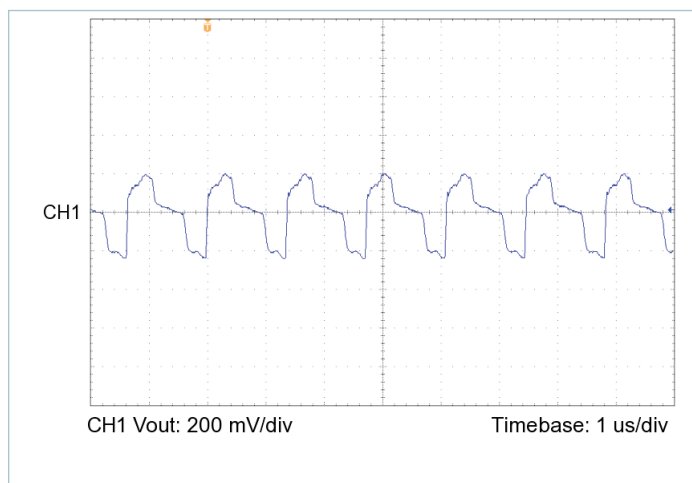
Figure 19 — Output voltage ripple, V_{IN} = 30\text{ V} , V_{OUT} = 12.0\text{ V} , C_{OUT\_EXT} = 1000\text{ μF} , R_{LOAD} = 0.896\text{ Ω}
