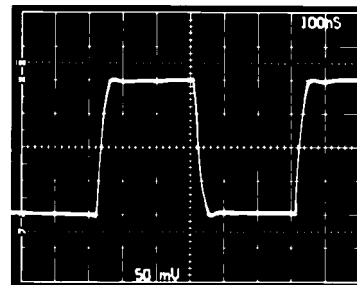
Figure 21c. Gain of 2 Follower Small Signal Pulse Response
