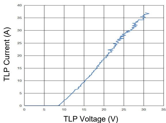
TLP Measurement of I/O to I/O
