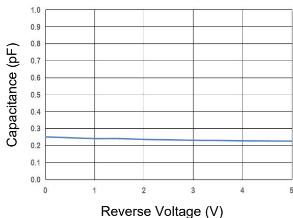
Capacitance vs Reverse Voltage IO to IO
