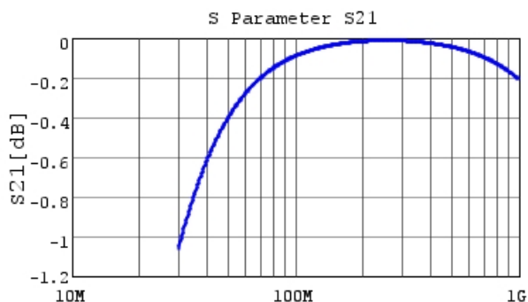
■ RHE5G2A101J0A2H03B S21 DCOV, 25degC
