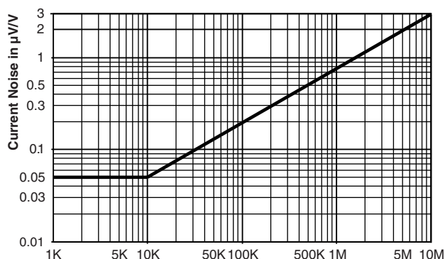
Current Noise
