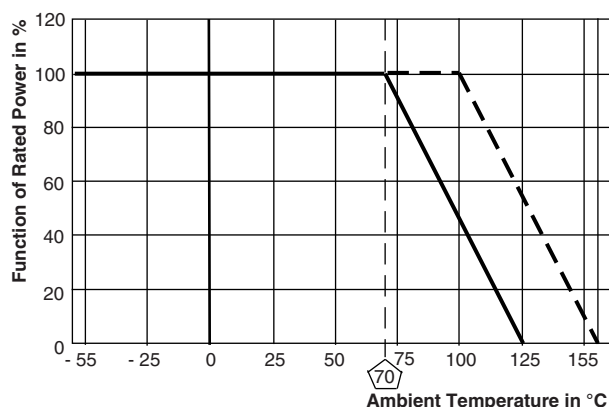
Derating
