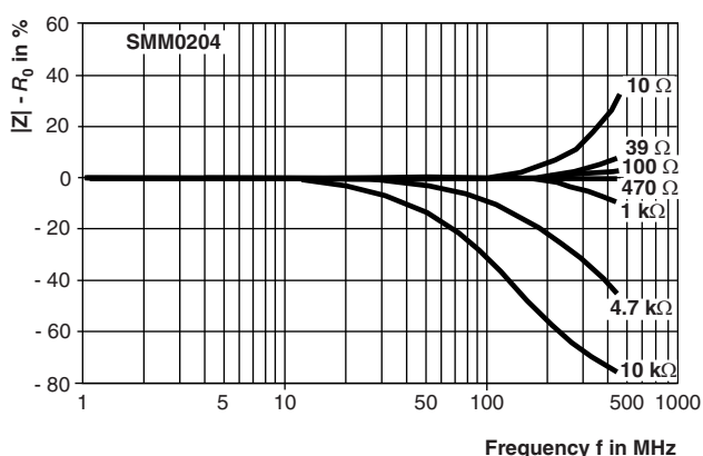
HF - Performance
