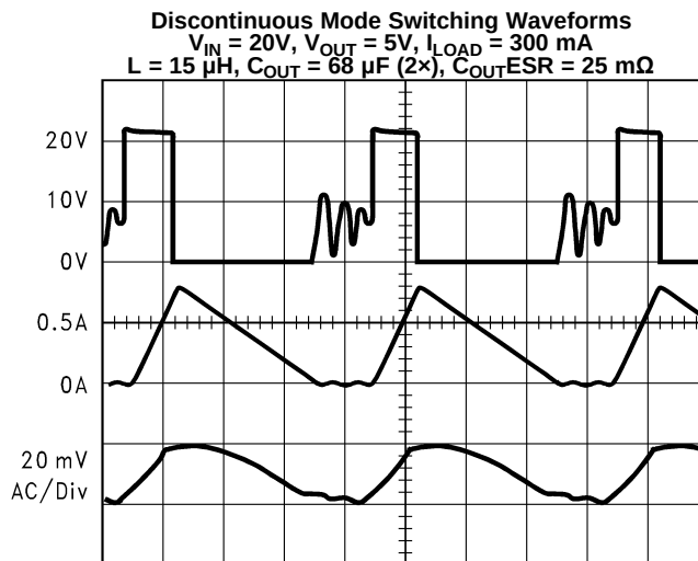
Figure 19. Horizontal Time Base: 1 \mu\text{s}/\text{div}
