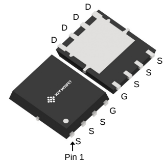
DFN5X6-8L (PDFN-8(5.8x4.9))
