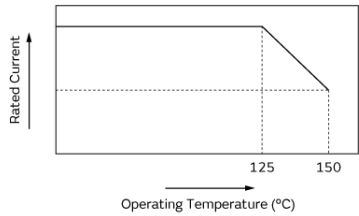
Derating of Rated Current
