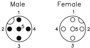
Contact Layout
