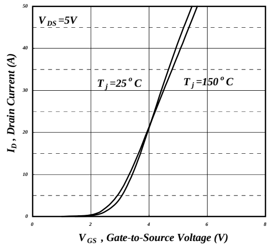
Fig 11. Transfer Characteristics
