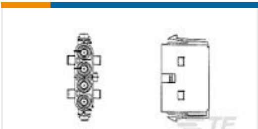
TE Part #794118-1 04P .156 MNL CAP PANEL MOUNT
