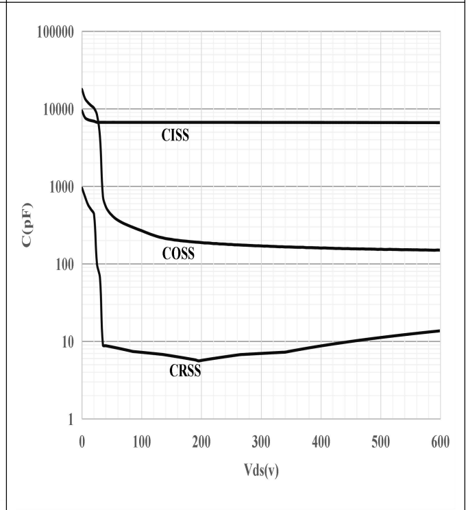
Figure 16: Typ. Capacitances
