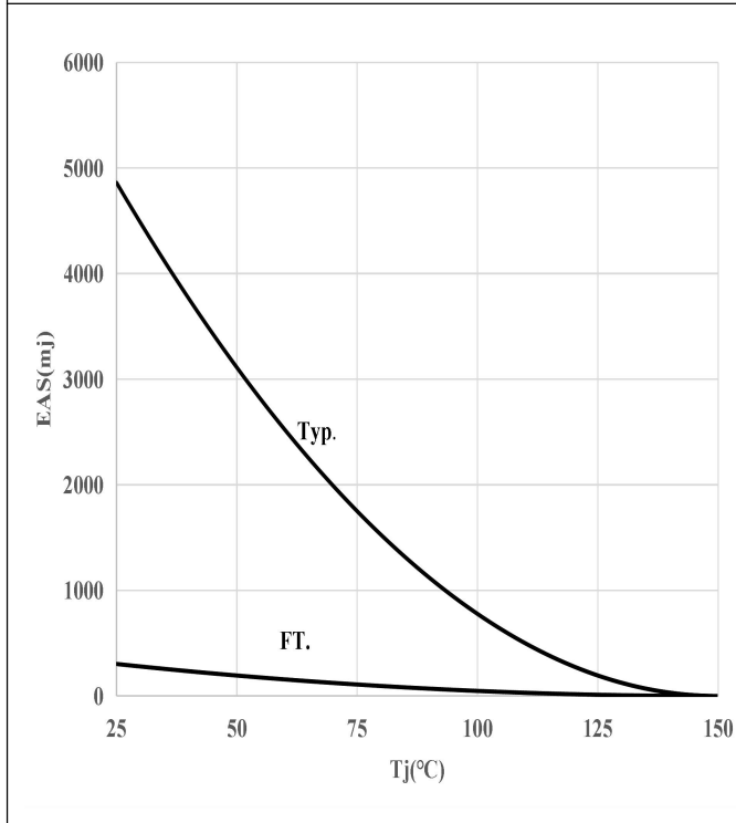
Figure 15: Avalanche Energy
