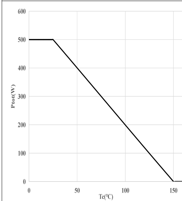
Figure 3: Power Dissipation
