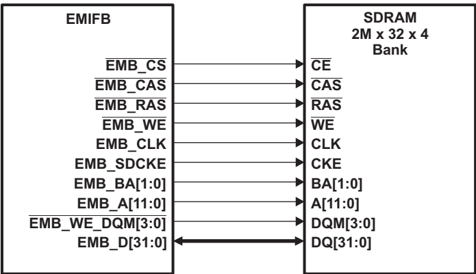
Figure 6-20. EMIFB to 2M × 32 × 4 bank SDRAM Interface
