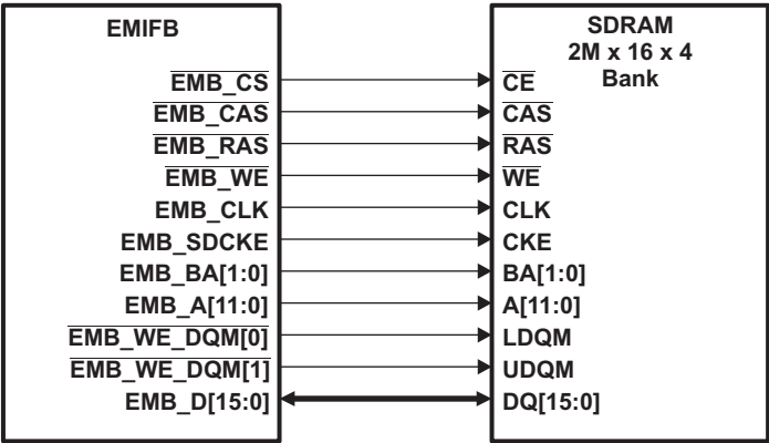
Figure 6-19. EMIFB to 2M × 16 × 4 bank SDRAM Interface
