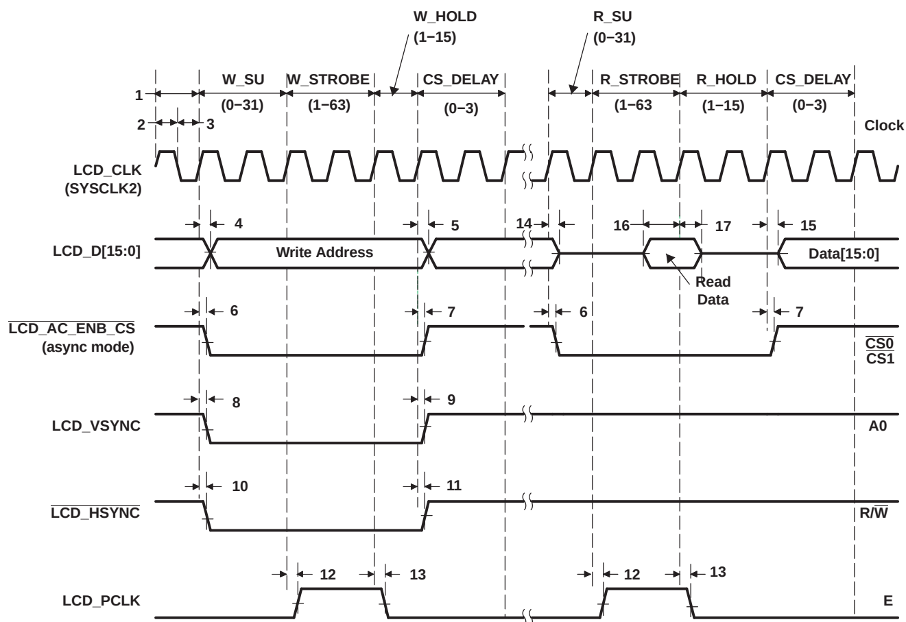
Figure 6-48. Micro-Interface Graphic Display 6800 Read
