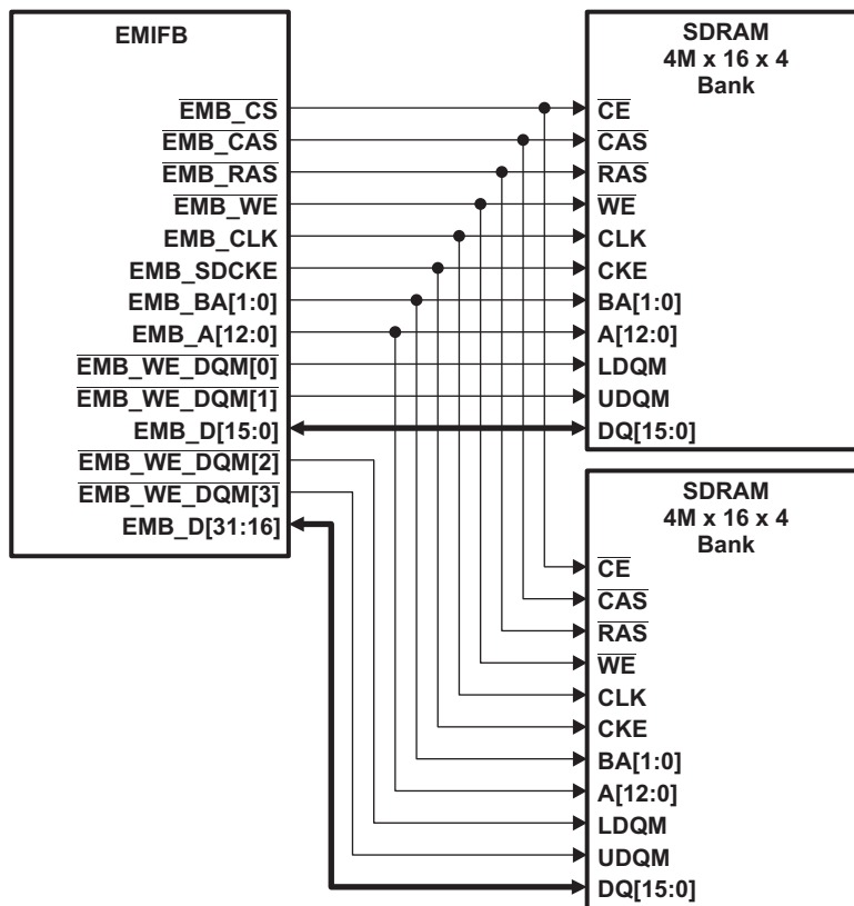
Figure 6-21. EMIFB to Dual 4M × 16 × 4 bank SDRAM Interface
