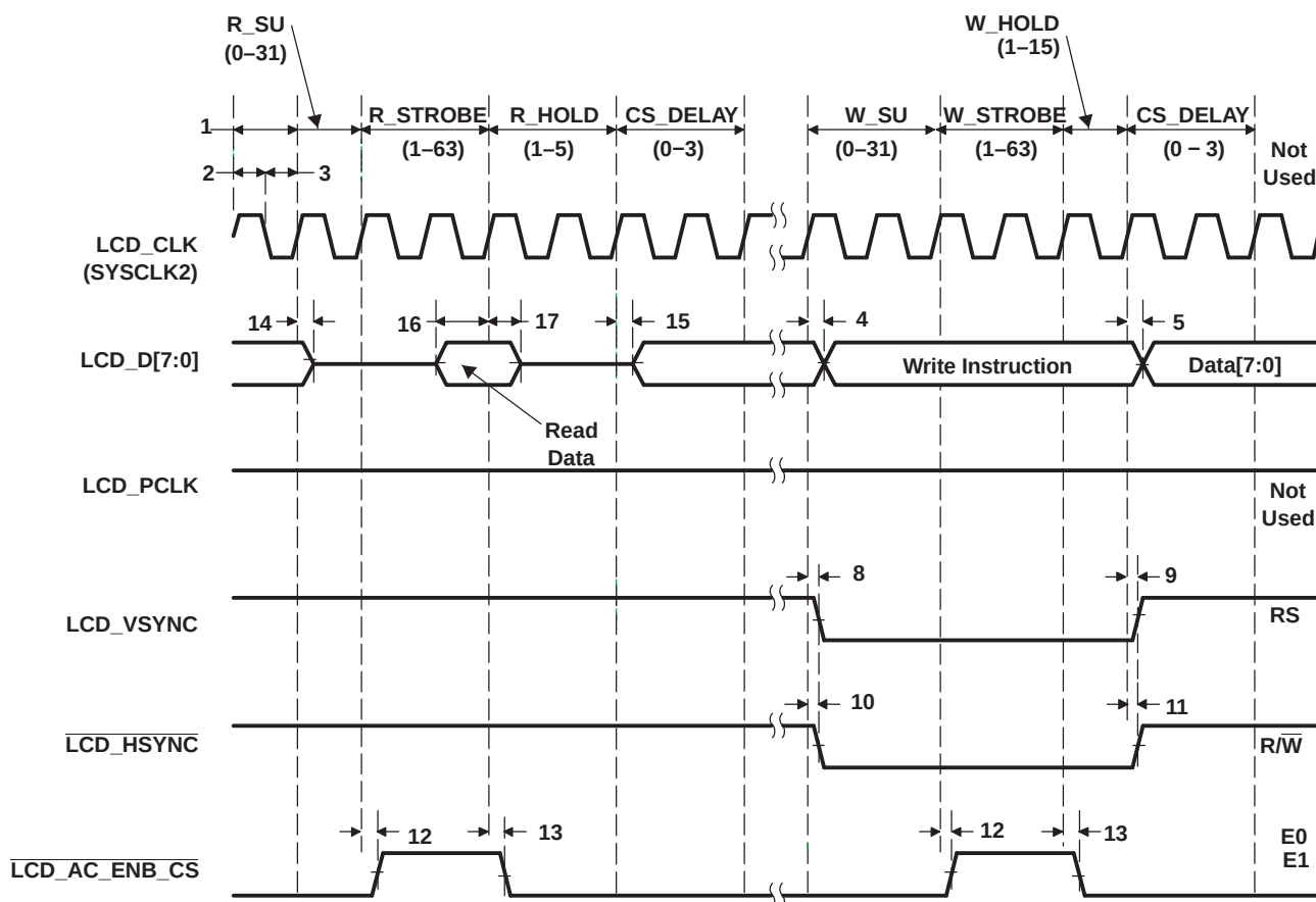
Figure 6-46. Character Display HD44780 Read
