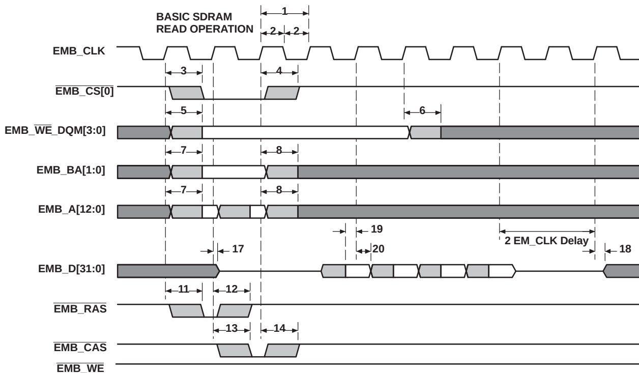
Figure 6-23. EMIFB Basic SDRAM Read Operation
