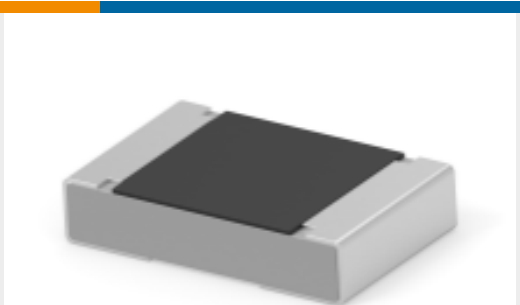
TE Part #3-2176523-7 3503G 2B 121R 1% 1K RL
