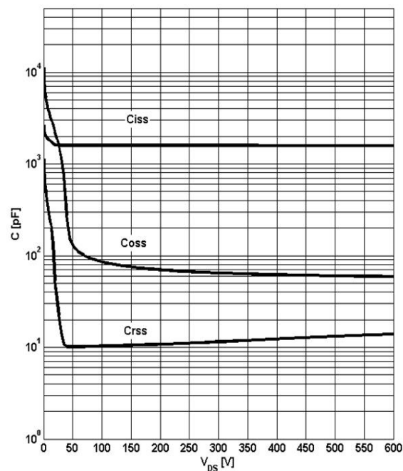
Figure 16: Typ. Capacitances
