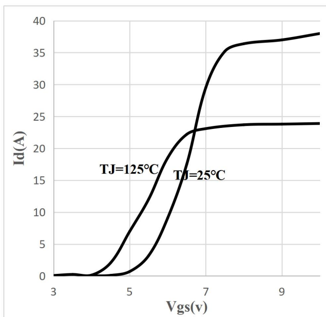
Figure 11: Typ. Transfer Characteristics
