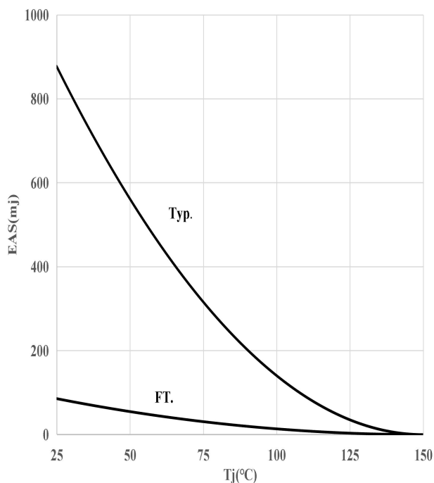
Figure 15: Avalanche Energy
