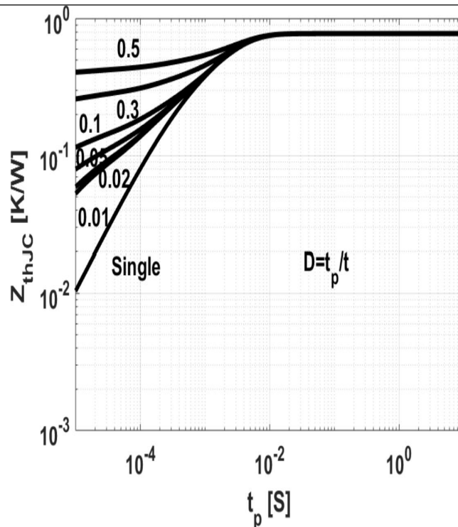
Figure 4: Max. Transient Thermal Impedance
