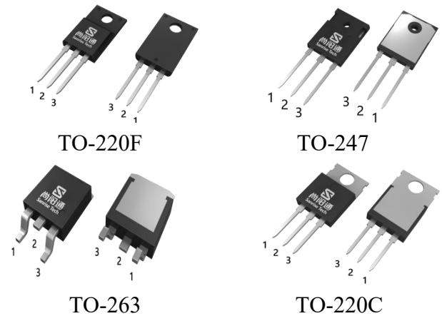
Figure 2 Package Types of SRC65R170B
