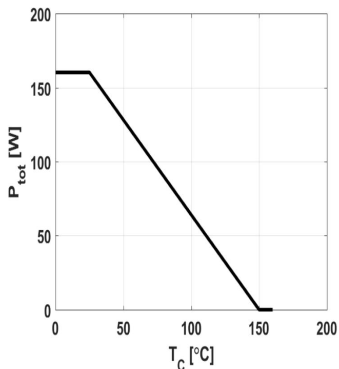
Figure 3: Power Dissipation
