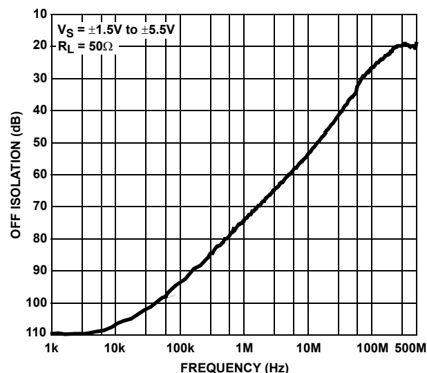
FIGURE 14. OFF ISOLATION
