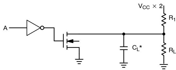
Figure 4. Test Circuit
