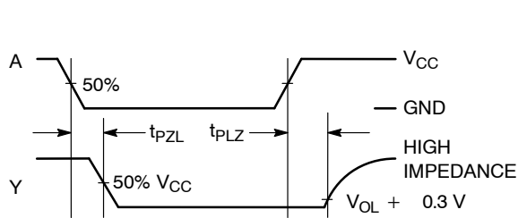
Figure 3. Switching Waveforms
