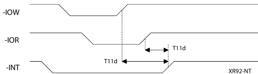
Figure 13: Interrupt Timing
