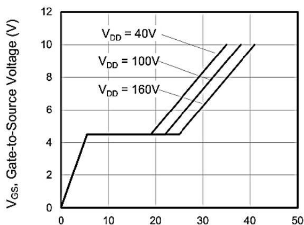
Figure 8. Gate Charge
