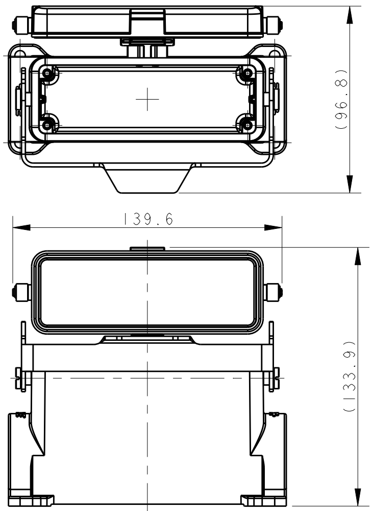
TYPE 6: HIGH BODY + SINGLE STEEL LOCKING + METAL PROTECTION COVER OTHER SPEC REFER TO TYPE 4
