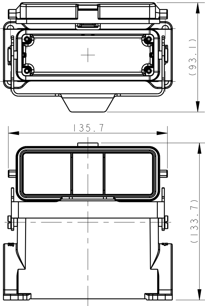
TYPE 5: HIGH BODY + SINGLE STEEL LOCKING + PLASTIC PROTECTION COVER OTHER SPEC REFER TO TYPE 4
