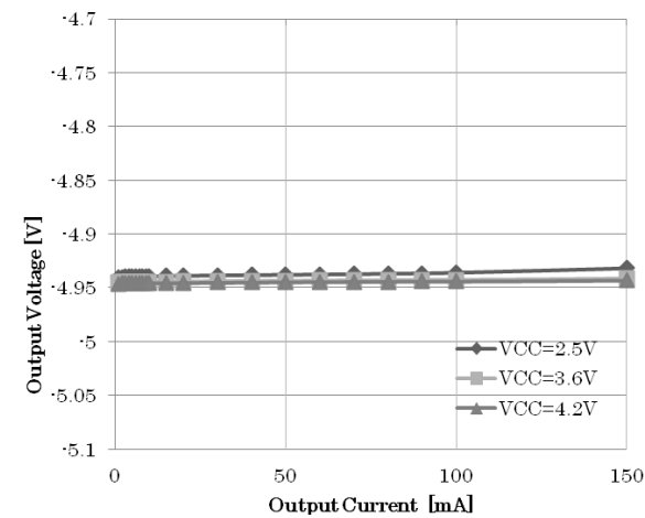
Figure 22. CH1 Output voltage vs Output Current
