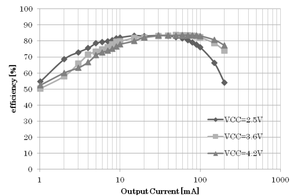
Figure 20. CH1 Power conversion efficiency vs output current
