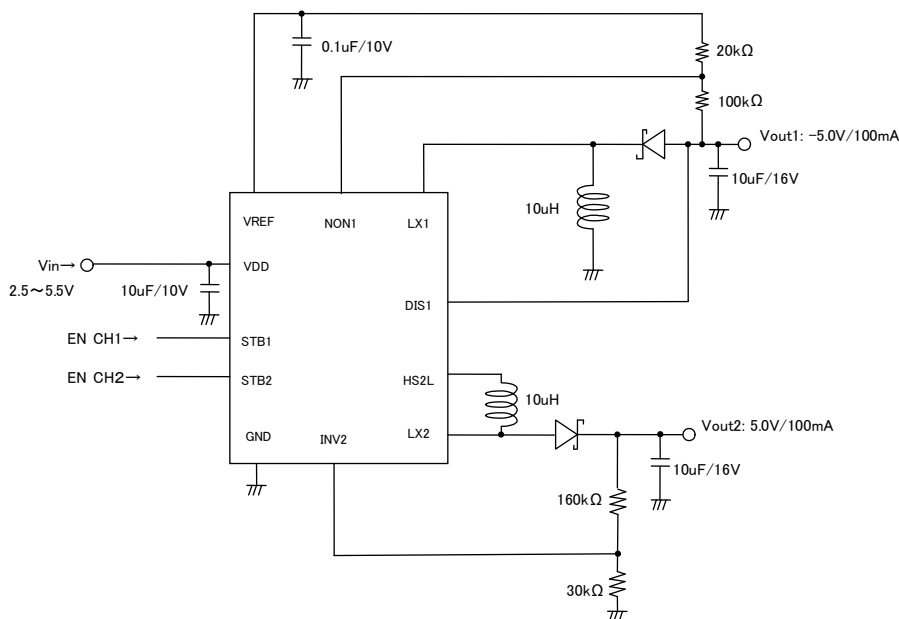
Figure 1. Application schematic
