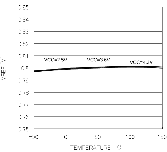
Figure 4. VREF vs temp
