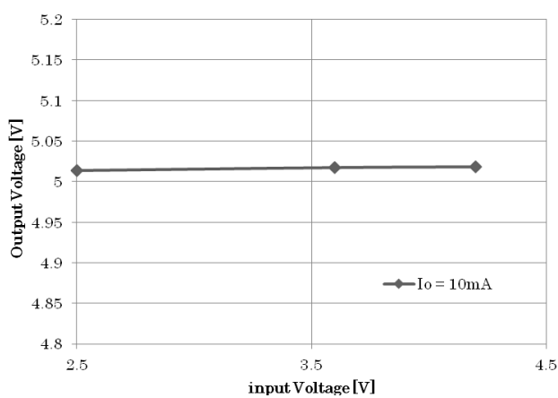
Figure 25. CH2 Output voltage vs Input voltage
