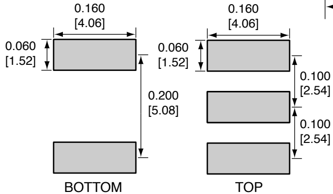
RECOMMENDED FOOTPRINT
