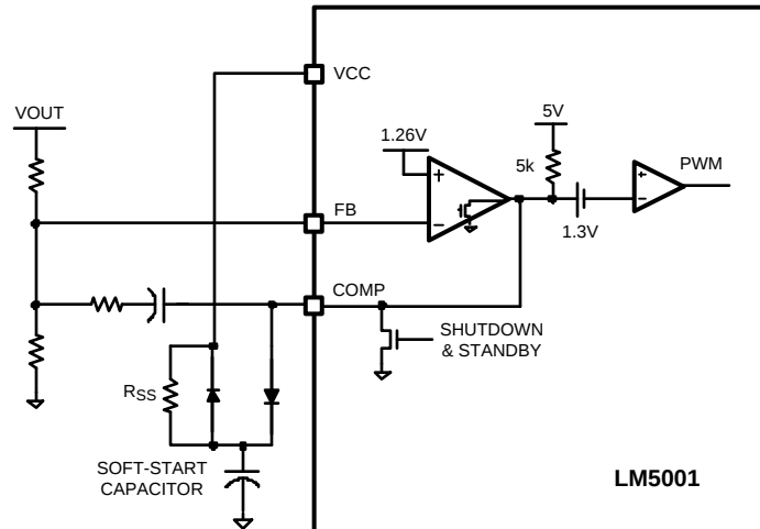
Figure 20. Soft-Start
