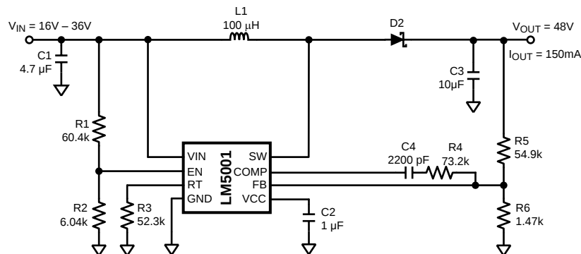
Figure 23. Boost
