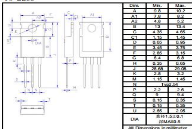
TO-220C
