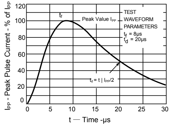
Figure.2 Pulse WaveForm-8/20μs
