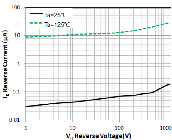
Figure 2. Reverse Characteristic(typ.)
