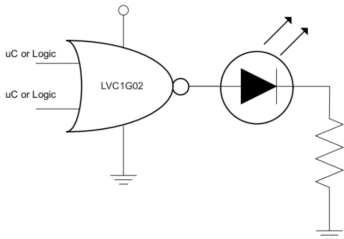
Figure 5.1: Application Schematic
