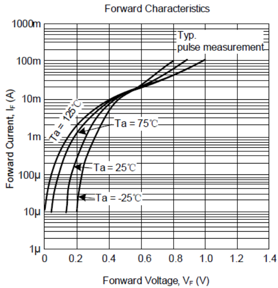
Fig.1 - Forward Characteristics
