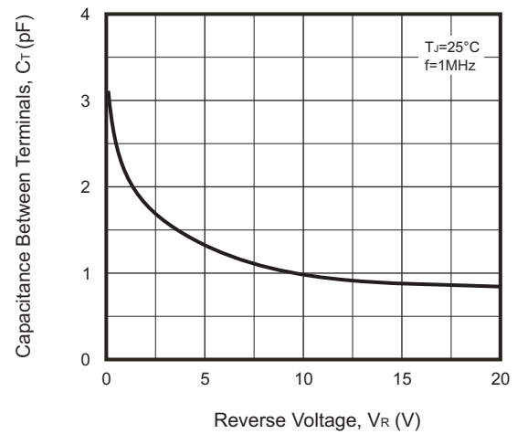
Fig.4 - Capacitance Characteristics
