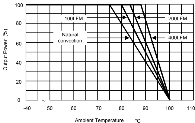
Derating Curve ( 3.3V, 5V & ±5V )
