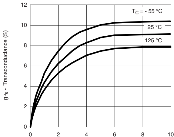
Transconductance
