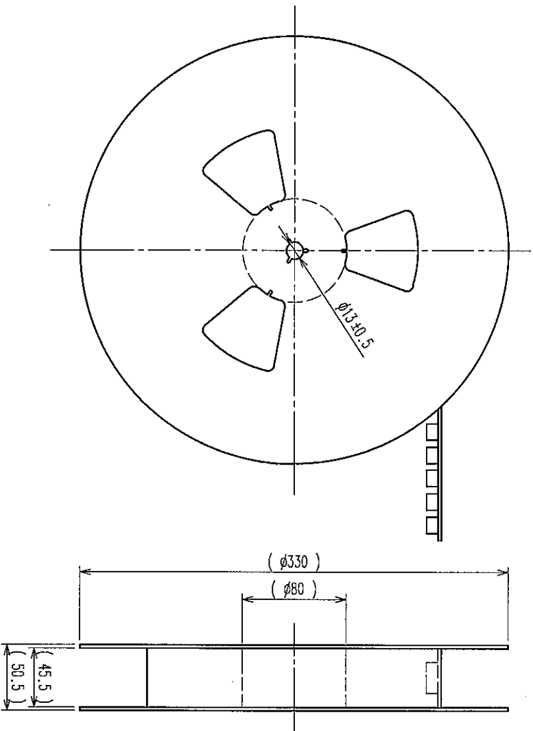
REELED DIMENSION (FREE)
