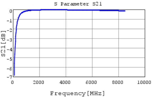
GRM0335C2A8R1BA01 S21 DCOV, 25degC
