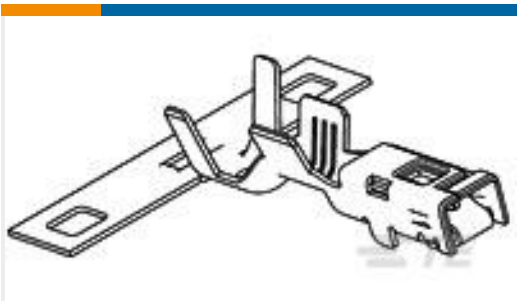
TE Part #1326032-6 2.8MM RECP,SEAL,12AWG
