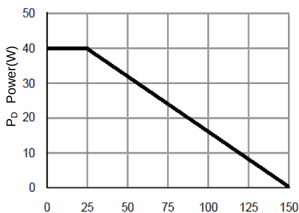
Figure 8 Power Dissipation
