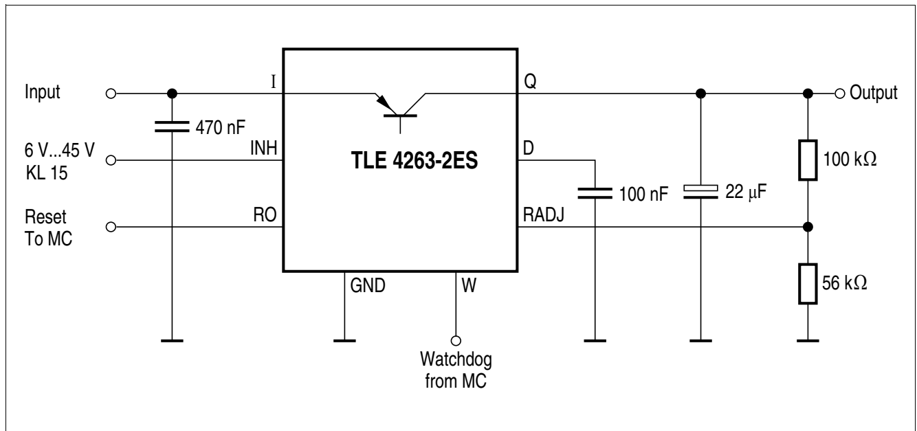
Figure 3 Application circuit
