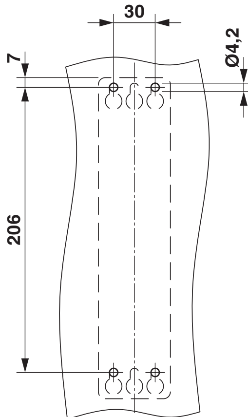
Drilling plan/solder pad geometry
