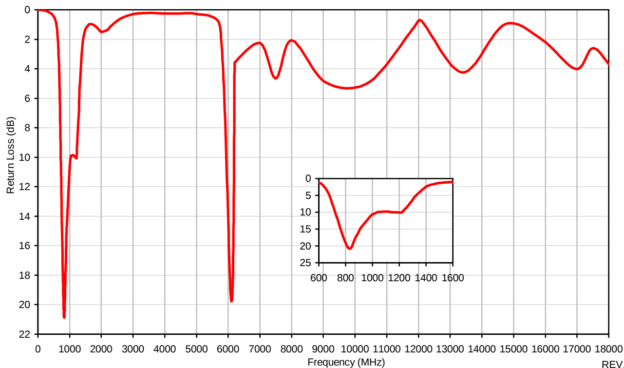
Return Loss
