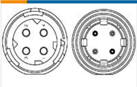
TE Part #1703780-1 4POS,PIN DIA 2.5,PIN HSG,ASSY
