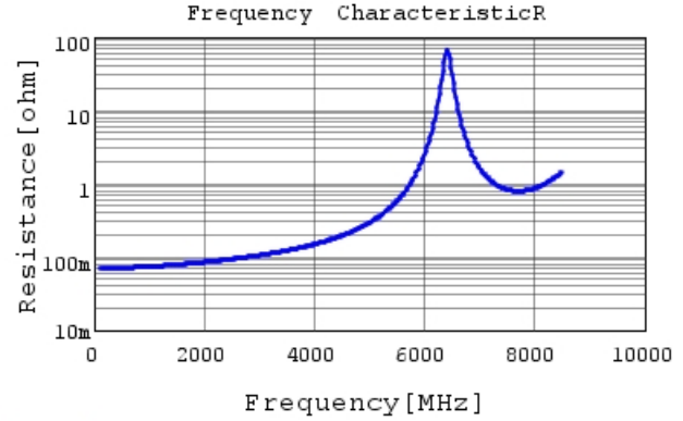
GQM1875G2E8R2WB12 R DCOV, 25degC
