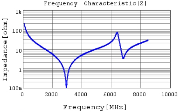
GQM1875G2E8R2WB12 |Z| DCOV, 25degC
