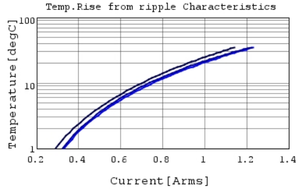
GQM1875G2E8R2WB12 Temp.rise 700MHz
